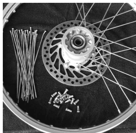
Left: Notice how the inner row of spokes on the far flange point clockwise, while the outer row points counter-clockwise. Also, see how their heads are recessed in the near side of this hub. Center: The partially installed spoke illustrates its specific features: The "head," "throat length" (distance it passes through the flange) and "angle" to match the direction to the rim. Right: The old wheel, half-way disassembled.
