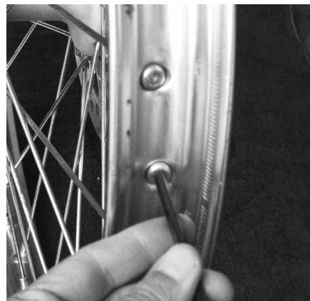
Left: A perfect fit between spoke wrench and nipple makes the job easy and... (Center) prevents this from happening. Not only is this nipple rounded, it's also become crushed against the spoke threads, making it doubly difficult to remove. Right: Once loosened "topside" with a wrench, nipples can be unscrewed easily from the other side.
